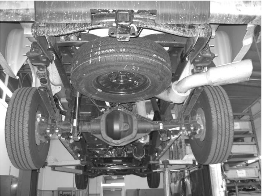
Figure 41- Single Exhaust
