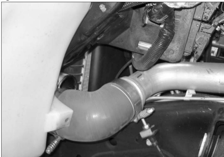
Figure 17 Drivers side boost hose
